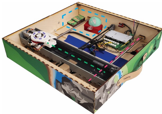
Figure 3: Travelling Forest hardware with x-axis (green), y-axis (pink), orientation theta (purple), and storage area (blue).
